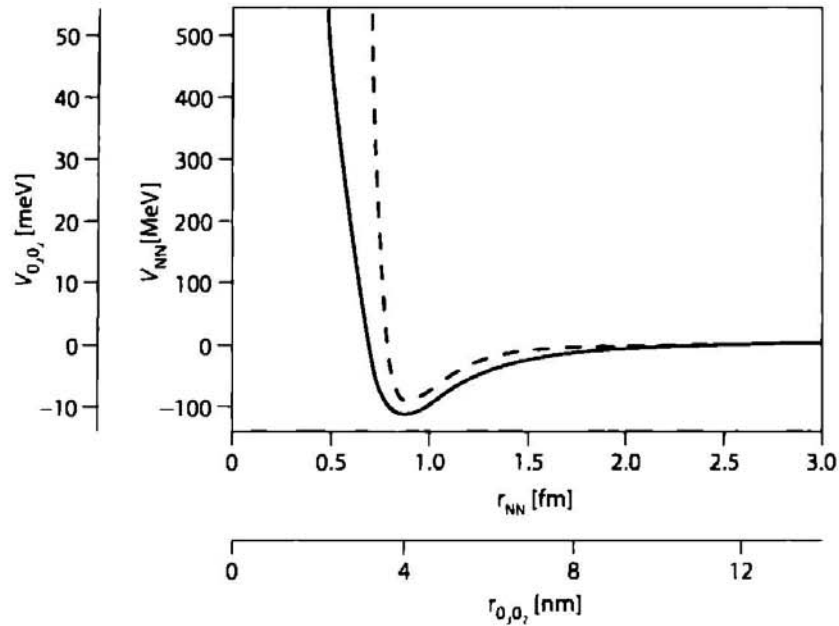
Figure 3.3 The NN potential in MeV (solid curve) in the ^1S_0 channel as a function of the NN distance in fm compared to the O_2 - O_2 molecular potential in MeV (dashed curve) as a function of the distance of separation in nanometers (outer axes).
