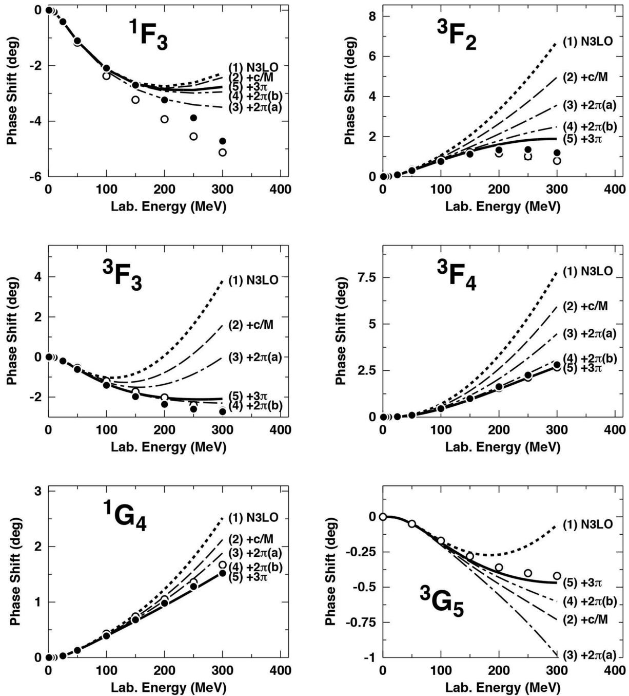
FIGURE 9 | Effect of individual fifth-order contributions to the neutron-proton phase shifts of some selected peripheral partial waves. The individual contributions are added up successively in the order given in parentheses next to each curve. In all cases an SFR cut-off \tilde{\Lambda} = 1.5 GeV is used. Curve (1) is N^3\text{LO} and curve (5) the complete N^4\text{LO} . The filled and open circles represent the results from the Nijmegen multi-energy np phase-shift analysis [93] and the VPI-GWU single-energy np analysis SM99 [91], respectively. Reprinted figure with permission from Entem et al. [46], copyright (2015) by the American Physical Society.
