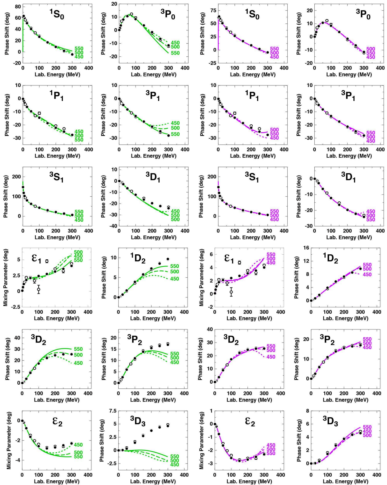
FIGURE 16 | Cutoff variations of the np phase shifts at NNLO (left side, green lines) and N^4 LO (right side, purple lines). Dotted, dashed, and solid lines represent the results obtained with cutoff parameter \Lambda = 450, 500 , and 550 MeV, respectively, as also indicated by the curve labels. Note that, at N^4 LO, the cases 500 and 550 MeV cannot be distinguished on the scale of the figures for most partial waves. Filled and open circles as in Figure 15 . Reprinted figure with permission from Entem et al. [37], copyright (2017) by the American Physical Society.
