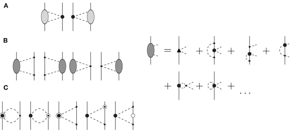
FIGURE 4 | N 4 LO 2π-exchange contributions to the NN interaction. The same notation as in Figure 3 is used. Open circles with a large solid dot inside refers to the 1/M_N corrections to vertices with two derivatives. Solid triangles represent vertices with index \Delta_i = 3 . The subleading one-loop \pi N amplitude is represented by a dark-shaded oval. Adapted figure with permission from Entem et al. [46], copyright (2015) by the American Physical Society. (A,B) Two-loop diagrams, and (C) relativistic corrections to one loop diagrams.
