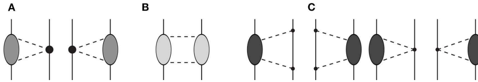
FIGURE 6 | N 5 LO 2 \pi -exchange contributions to the NN interaction. There are three classes of diagrams. Class (A) is obtained from the subleading one loop \pi N amplitude folded with the subleading \pi\pi NN vertex proportional to c_i . Class (B) is obtained from the leading one-loop \pi N amplitude folded by itself. Class (C) is obtained from the leading two-loop \pi N amplitude (represented by a black oval) with the tree-level \pi N amplitude. Other notation as in Figure 6 . Adapted figure with permission from Entem et al. [48], copyright (2015) by the American Physical Society.
