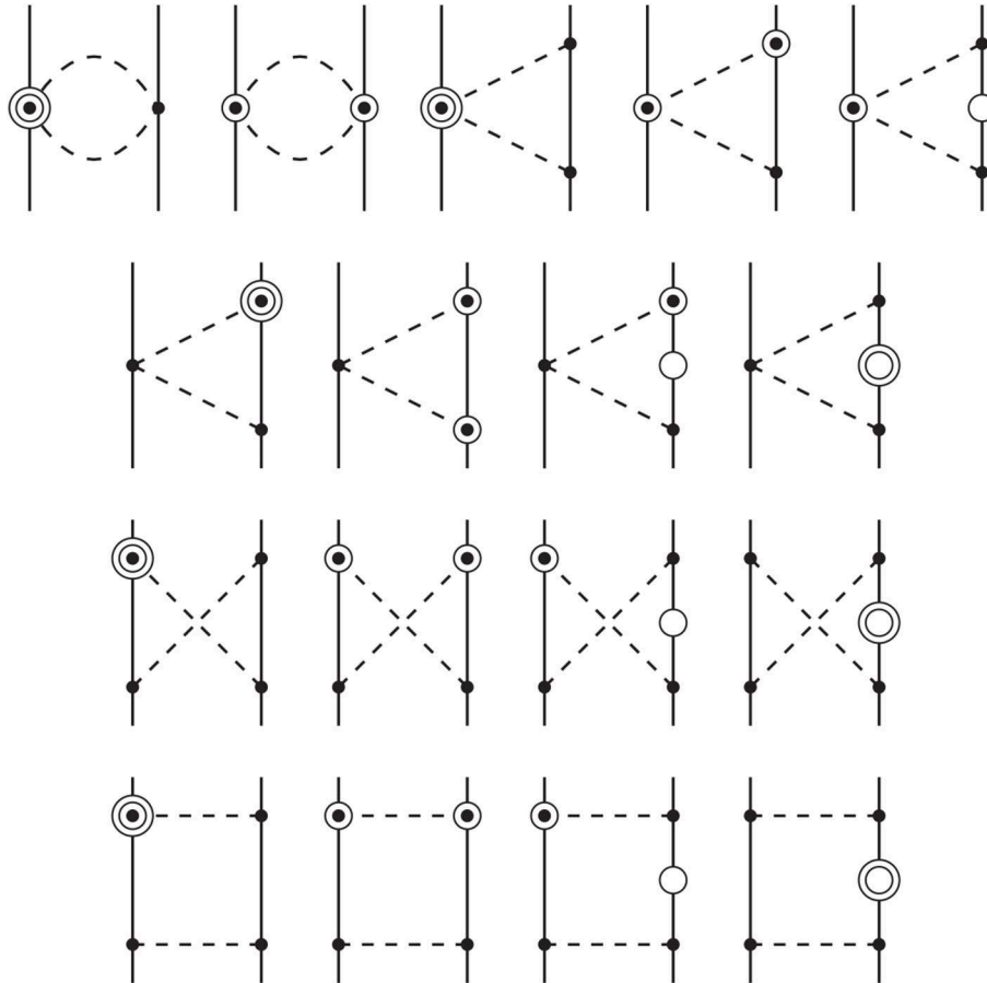
FIGURE 7 | N 5 LO 2 \pi exchange contributions to the NN interaction coming from 1/M_N^2 corrections to the NLO chiral 2 \pi -exchange diagrams. Notation as in Figure 3 . Two open circles refers to 1/M_N^2 corrections to propagators and vertices as in the case of one open circle. Reprinted figure with permission from Entem et al. [48], copyright (2015) by the American Physical Society.
