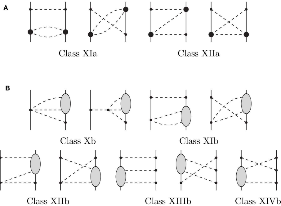
FIGURE 8 | N 5 LO 3π-exchange contributions to the NN interaction. (A) Diagrams proportional to c_i^2 . (B) Diagrams involving the one-loop \pi N amplitude. Notation as in Figure 3 . Reprinted figure with permission from Entem et al. [48], copyright (2015) by the American Physical Society.
