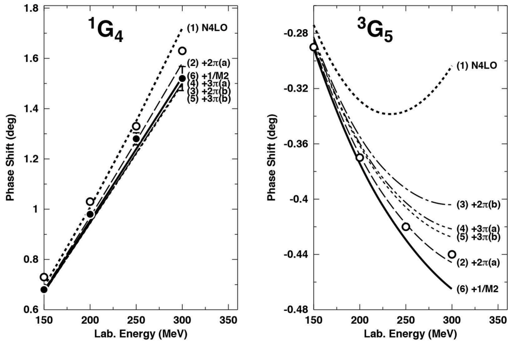
FIGURE 12 | Effect of individual N^5 LO contributions to the neutron-proton phase-shifts of two G waves. Contributions are added up successively starting from the N^4 LO result (1) to the final N^5 LO result (6). A SFR cutoff \tilde{\Lambda} = 800 MeV is used. The filled and open circles represent the results from the Nijmegen multienergy np phase-shift analysis [93] and the GWU np analysis SP07 [94], respectively. Reprinted figure with permission from Entem et al. [48], copyright (2015) by the American Physical Society.
