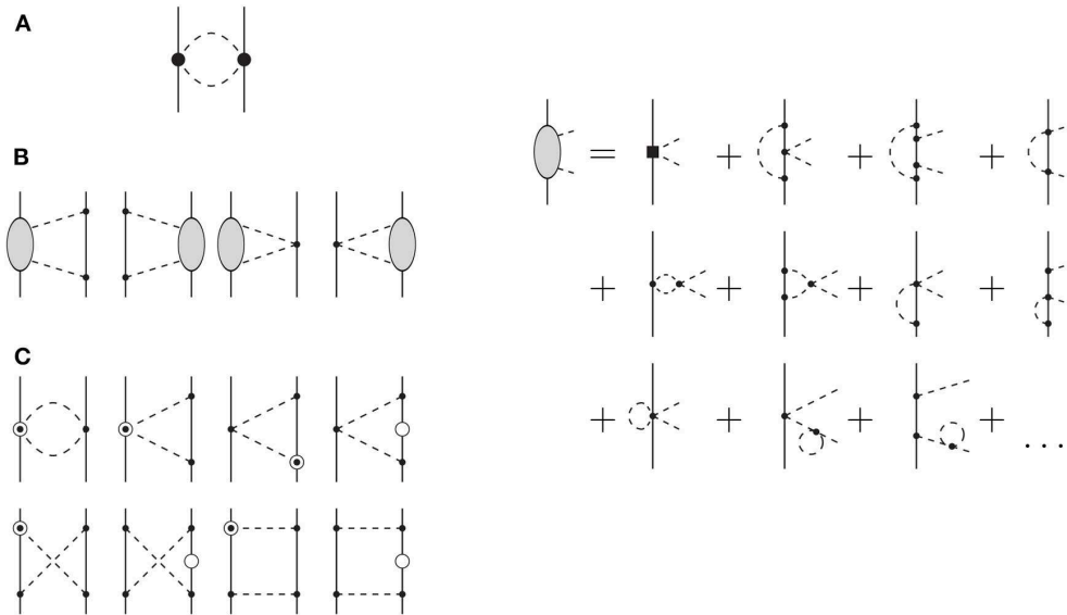
FIGURE 3 | N 3 LO 2π-exchange contributions to the NN interaction. The same notation as in Figure 2 is used. Solid squares represent vertices with index \Delta_i = 2 . Open circles and open circles with a dot inside are relativistic 1/M_N corrections to propagators and the vertex with one derivative, respectively. The leading one-loop \pi N amplitude is represented by a shaded oval. Adapted figure with permission from Entem et al. [46], copyright (2015) by the American Physical Society. (A) Football diagram, (B) two-loop diagrams, and (C) relativistic corrections to one loop diagrams.
